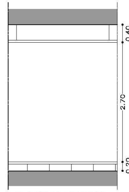
4. DETAIL SECTION - FLOOR HEIGHTS
