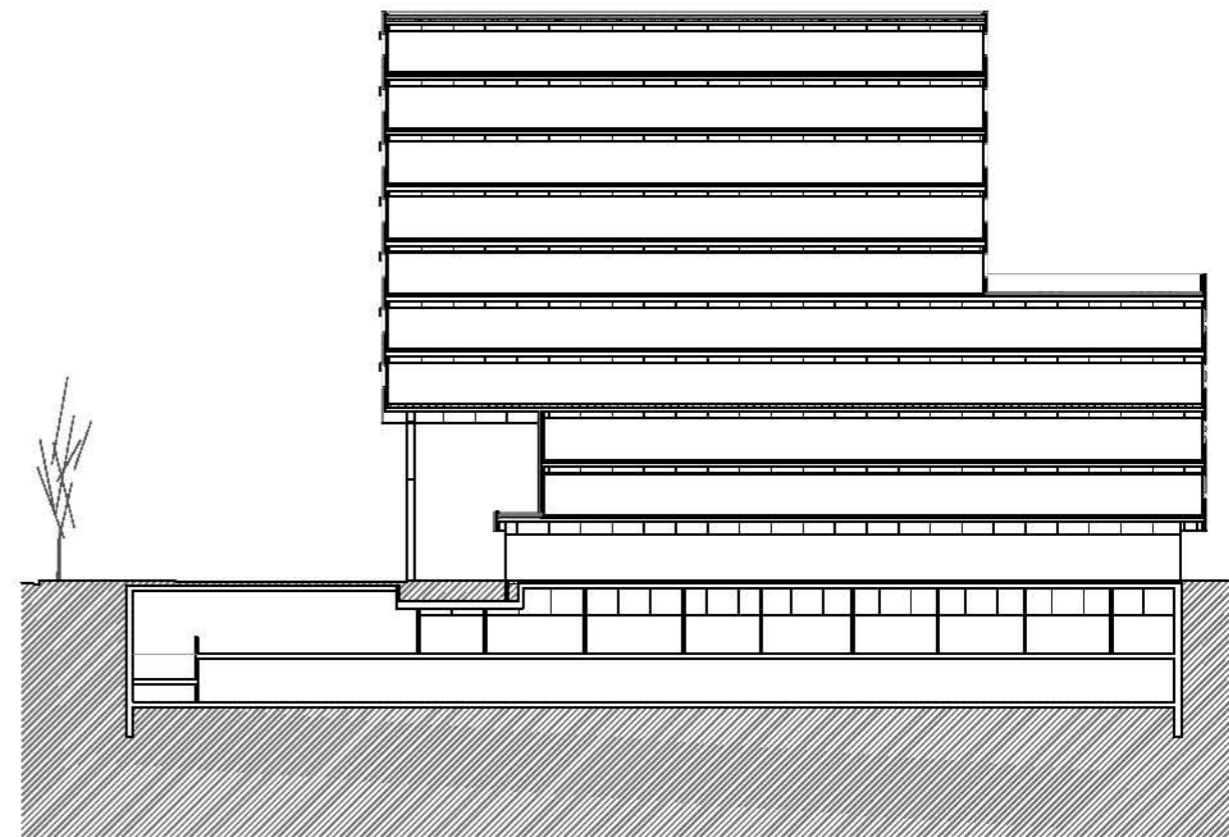
3. INTERIOR SECTION - BUILDING C
