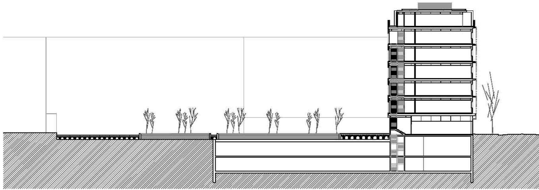
1. INTERIOR SECTION - CARRER PALLARS
